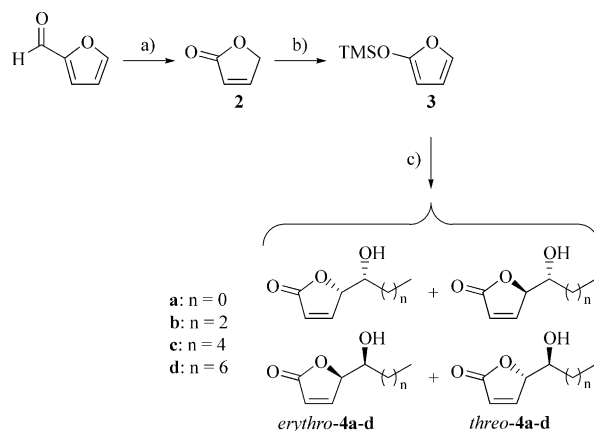
Scheme 4. (a) HCOOH, H 2 O 2 , Na 2 SO 4 , K 2 CO 3 , H 2 O, CH 2 Cl 2 , reflux to rt; then Et 3 N, toluene, rt; (b) TMSCl, Et 3 N, 0°C to rt; (c) CH 3 (CH 2 ) n -CHO, TESOTf, CH 2 Cl 2 , –78 °C; then 1M HCl, rt.
