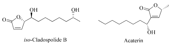
Scheme 2. Natural products iso -cladospolide B and acaterin.
