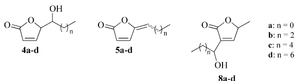
Scheme 3. Target scaffolds, derived from iso -cladospolide B ( 4a–d and 5a–d ) and acaterin ( 8a–d ), respectively.
