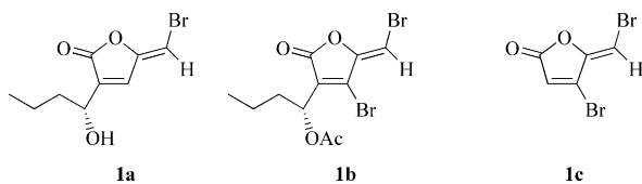
Scheme 1. Structures of some naturally occurring halogenated furanones, 1a–b , and a synthetic analogue 1c , all antagonists in quorum sensing systems.
